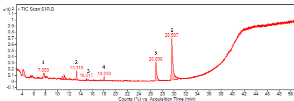
Figure 2: Chromatogram of hexane extract of H. formicarum tubers
